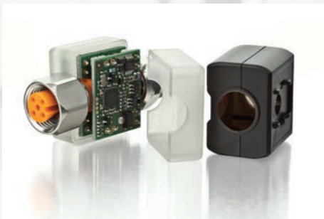
Sensor in plastic housing
